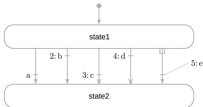
Figure 17.1: Recommended layout of a simple state machine. For the 5 transitions, the settings are as follows, from left to right: immediate = true, false, true, false, true; reset = true, true, false, false, true; synchronize = false, false, false, false, true; priority = 1, 2, 3, 4, 5.
